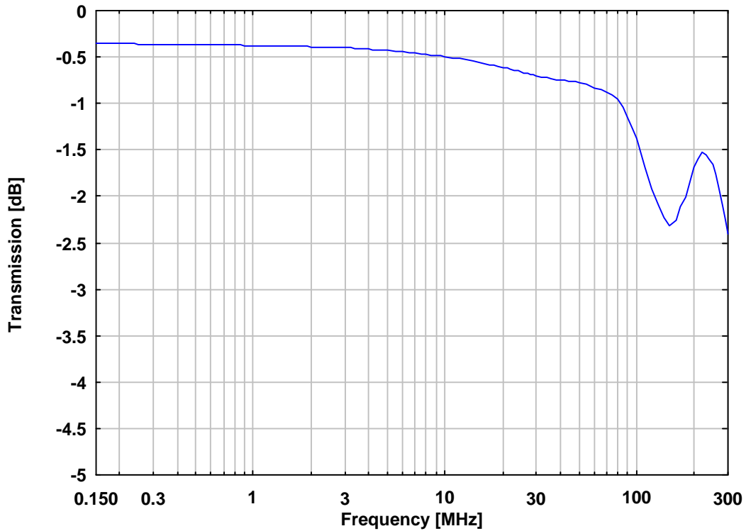
Transmission Differential Mode Signal AE-EuT
