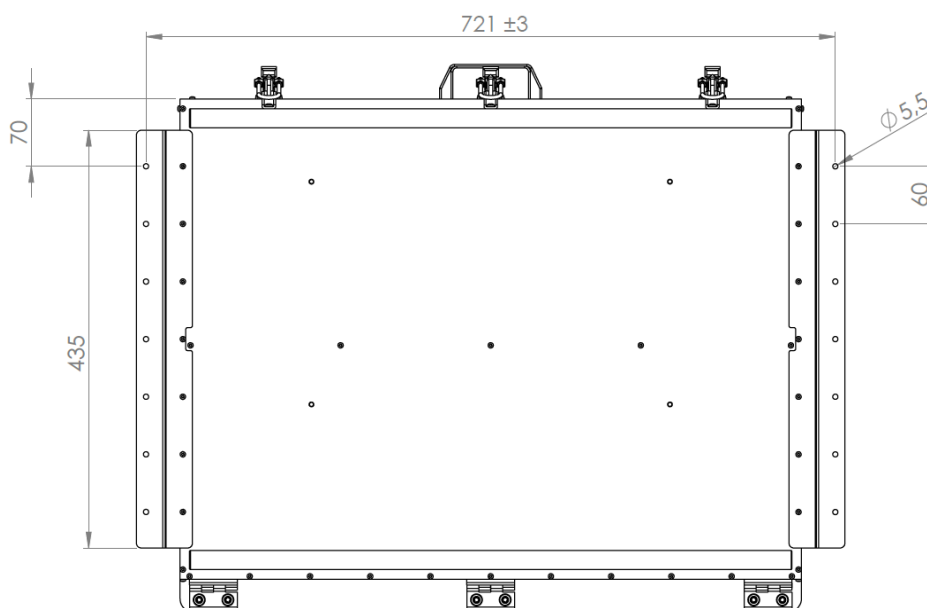
Montageposition der Erdungsschiene Position of mounting holes for Ground-Connection
